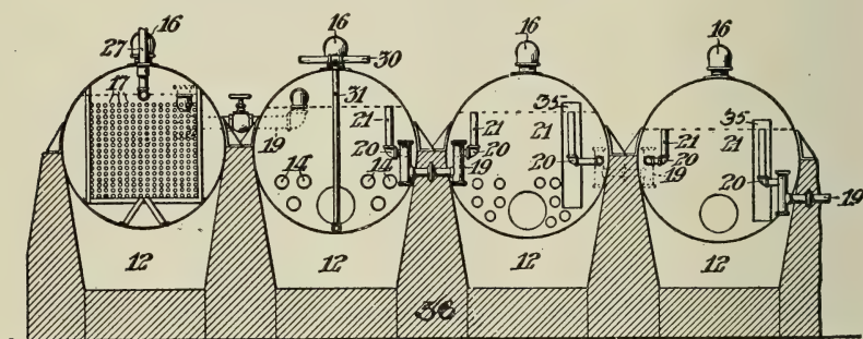
FIG. 109.—Livingston Apparatus for Continuous Distillation of Petroleum.
